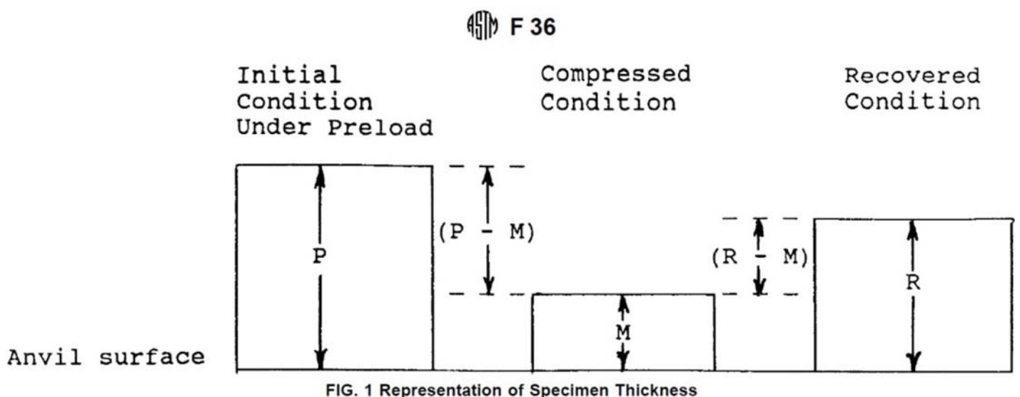
Figure 2: ASTM F 36 – compression/recovery (source: ASTM F 36).
