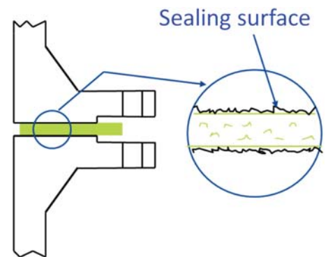
Figure 1: Surface structure of the sealing surface.
